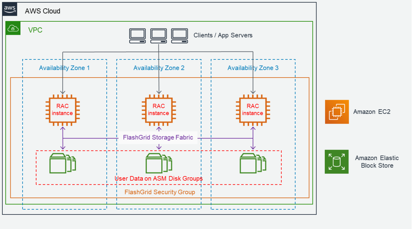
FlashGrid Cluster Network Diagram
